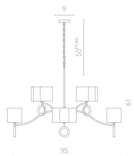
1 4069/02 LM-8 ∅95 | ↑61 | 50 max ⚡ 8x40W E14
