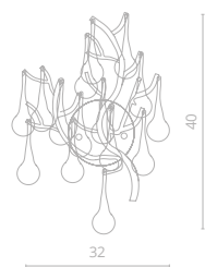
3 3132/01 AP-3 ↔32 | ↗18 | ↓40 ⚡ 3x40W G9
