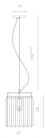
5 3001/01 SP-1 ∅22 | ↓28 | 100 max ⚡ 1x75W E27
