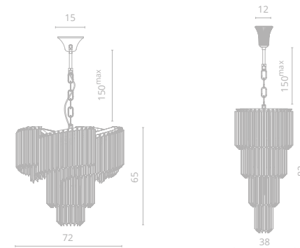
3 1681/01 LM-9 ∅72 | 165 | 150 max ⚡ 9x60W E14 ⚙ 29 4 1681/01 SP-9 ∅38 | 182 | 150 max ⚡ 9x60W E14 ⚙
