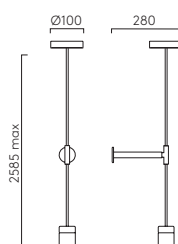
PENDANT SUSPENSION KIT 3 / KNURLED
