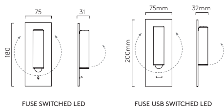
FUSE SWITCHED LED
