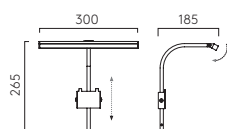
MONDRIAN FRAME MOUNTED 300
