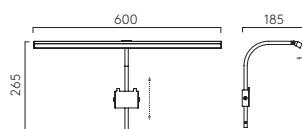
MONDRIAN FRAME MOUNTED 600
