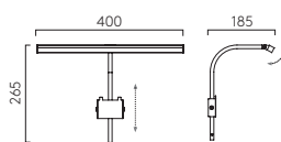
MONDRIAN FRAME MOUNTED 400
